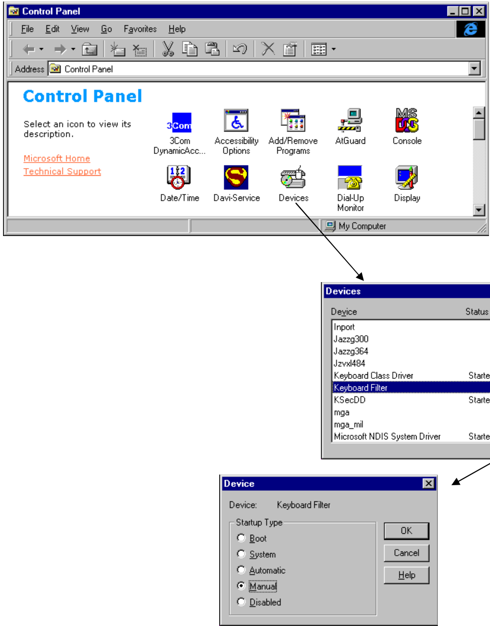
Figure 2.10. Start-up priority of the keyboard filter device driver for NT4.
